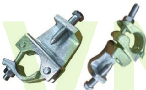
GIRDER FIX / SWIVEL DROP FORGED COUPLER
