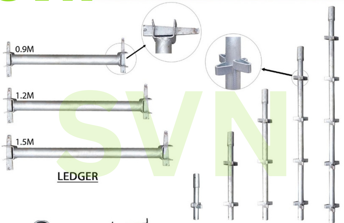
KWIKSTAGE STANDARD
