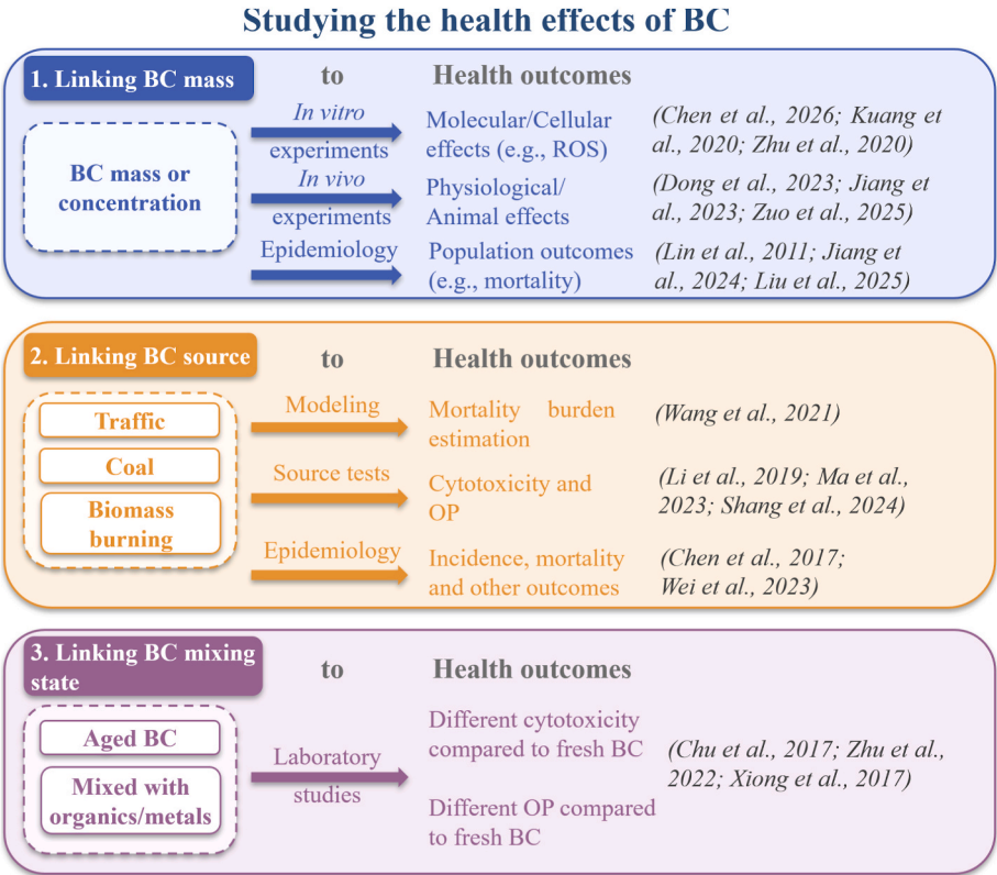
Fig. 7. Examples of studies linking BC mass, BC sources, and BC mixing states to health outcomes in China. Details are provided in Sections 6.1, 6.2, and 6.3.
