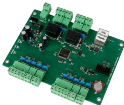
SKN-DC-8411 2 Door / 4 Reader Communication : LAN Register Cards : 42000 Record Capacity : 200000 Camera can be Integrate Input: Wiegand26/34
